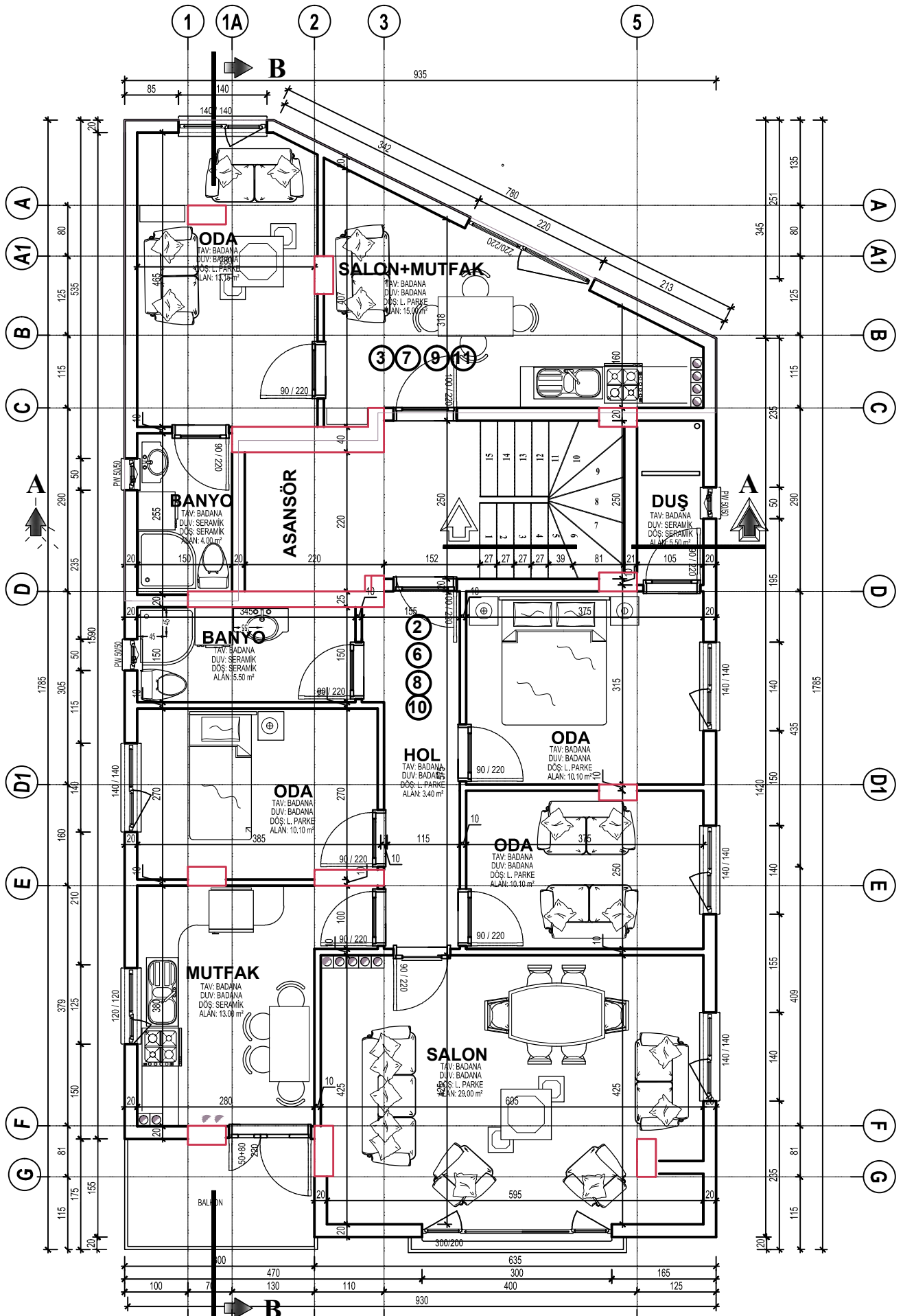
TADILATLI 2. BODRUM,ZEMİN,1.,2., KAT PLANI Ö:1/50
